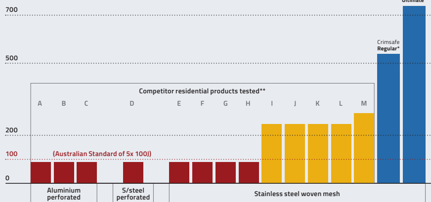
Graph prepared by Crimsafe on tests conducted by The University of Queensland 2017.
